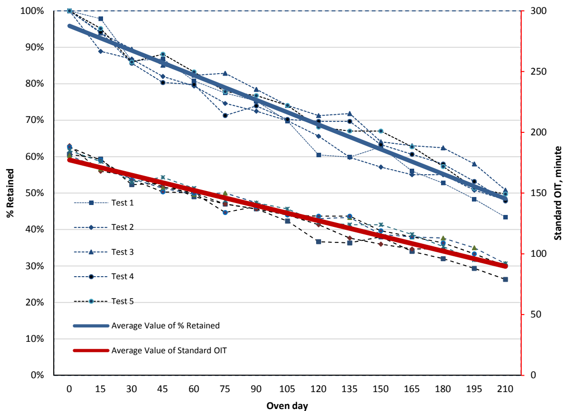
Trend Chart of Standard OIT Decay under 85 °C Oven
