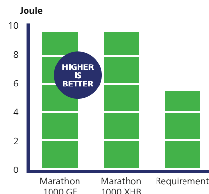
TEST RESULTS: IMPACT RESISTANCE
