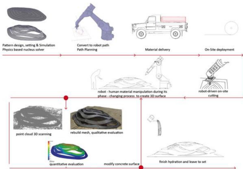
Figure 11: Path planning workflow and feedback loop.
