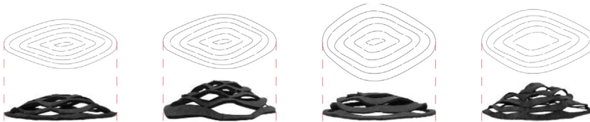
Figure 8: Comparison of geometric differences in the 3D pop-up surfaces, product of changes in boundary conditions and cutting patterns.
