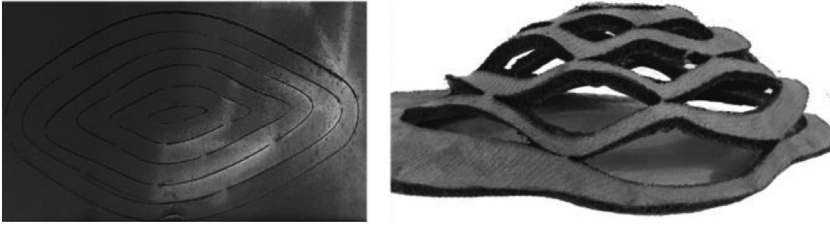
Figure 4: Left: 2D pattern laser cut in concrete canvas. Right: Popped-up concrete canvas shell prototype.
