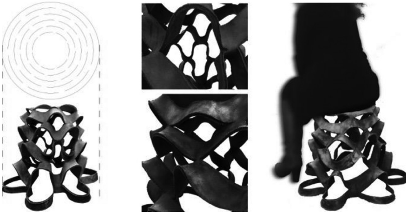
Figure 12: Left: Pattern and resultant pop-up geometry. Middle: Concrete details. Right: Live load testing to calibrate with structural assumptions.
