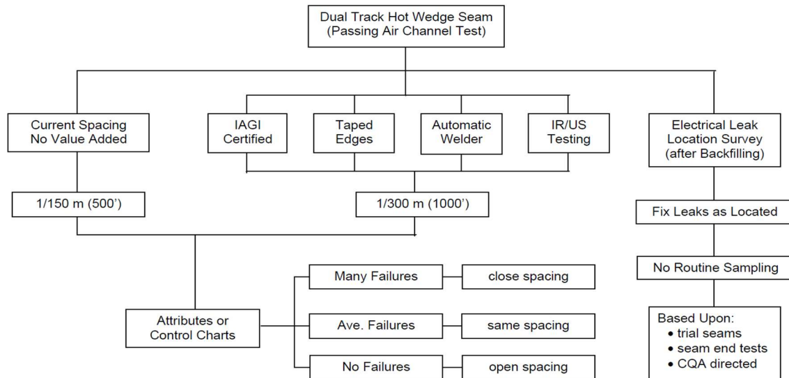
Figure 1: Suggested Strategy for Destructive Test Sampling (from GRI White Paper #3 by Koerner & Koerner, 2003).
