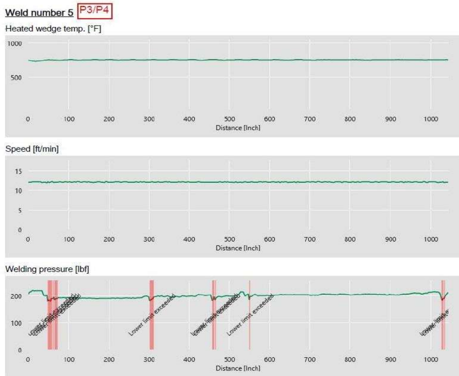
Figure 8: Data Acquisition Welding Report – Graphical Report showing the temperature, speed, and pressure plotted versus the data measurement position (distance).
