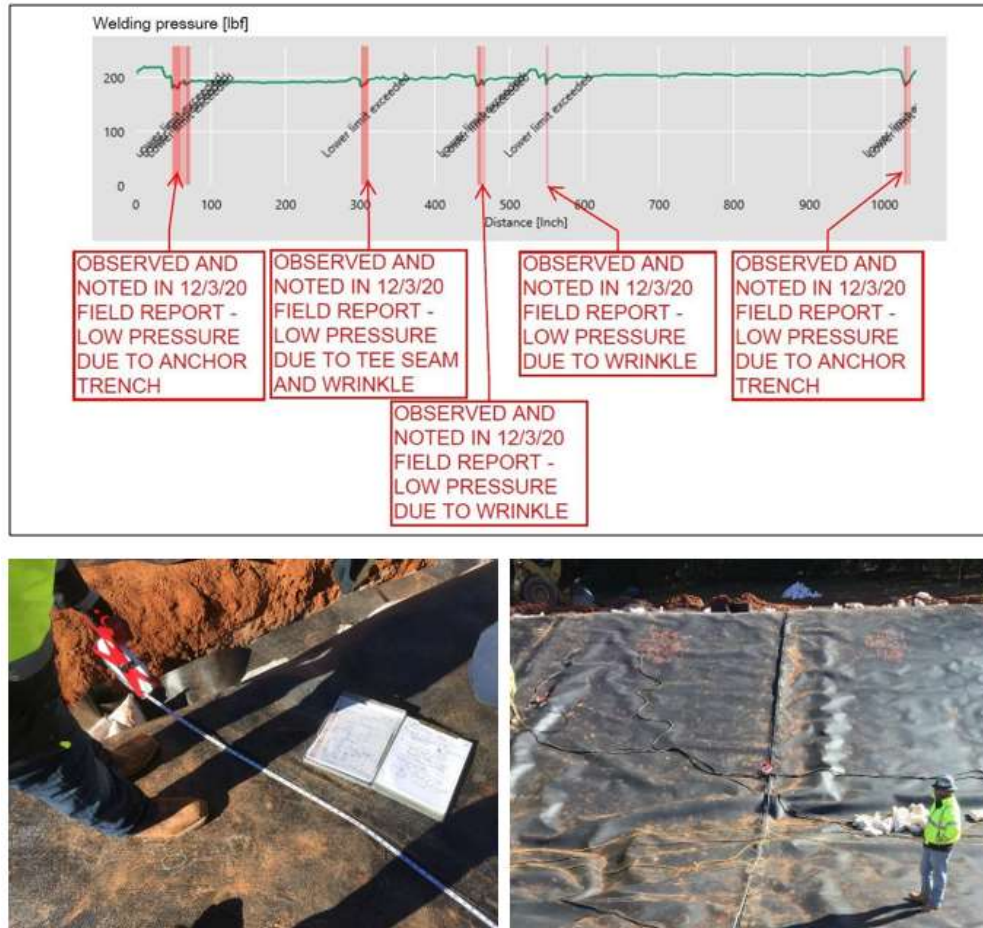
Figure 10: Top shows graphical pressure report of out of tolerance pressure readings with CQA location descriptions and explanations. Photo on the bottom left shows a typical anchor trench location recorded with low pressure; photo on the bottom right shows the location of a wrinkle that recorded low pressure.
