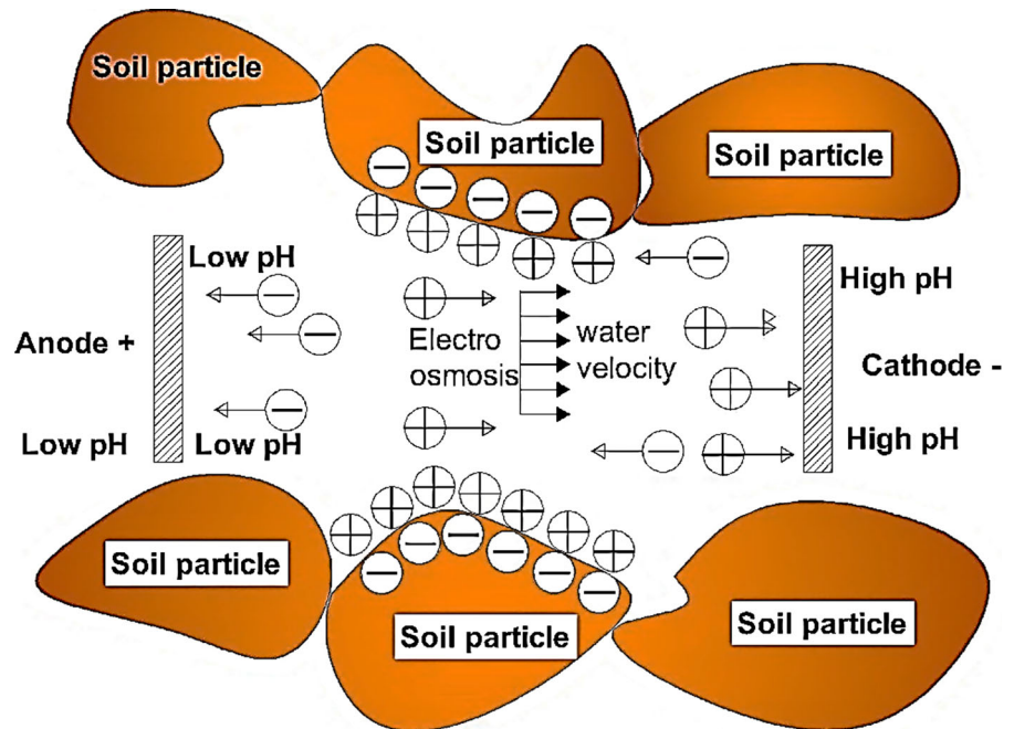
Fig. 2 Conceptual of movements in electrokinetic
