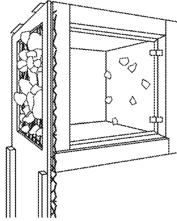
Side elevation showing aggregate retained on grid after test and also showing the small amount of aggregate that has fallen through the grid
