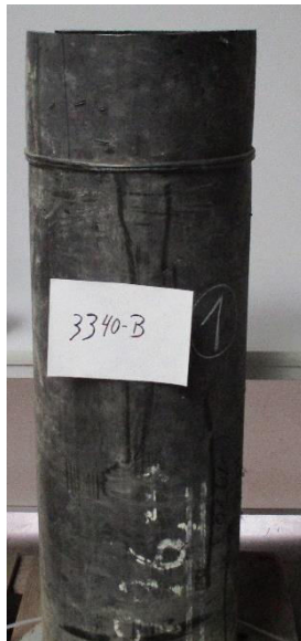
Fig. 3: Test sample
