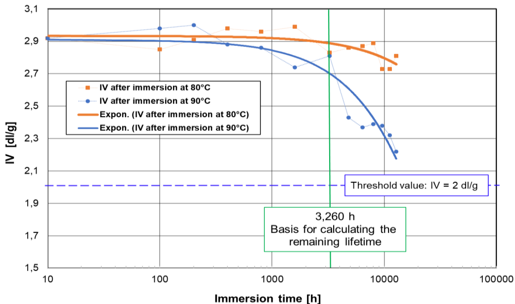
Fig. 7: Change in the mean viscosity expressed as Intrinsic Viscosity IV vs. immersion time
