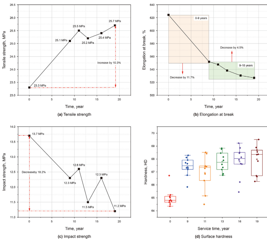
Fig. 4. Mechanical properties of pipelines with different service times.
