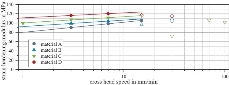
Fig. 3. Influence of the cross-head speed on the strain hardening modulus for different PE materials tested at a temperature of 23 °C. [13]
