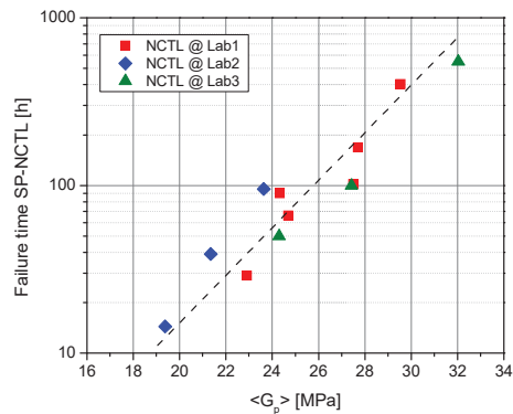
Fig. 6. Strain hardening modulus <G p
