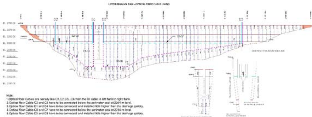
Fig. 11 : Position of the Optical Fiber Cable along the entire periphery of the dam
