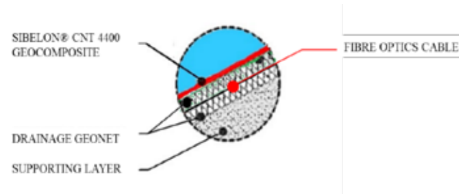
Fig. 3 : Cross section of the position of the fibre optics cable within the sandwich composed of the GM and the upstream face of the structure.
