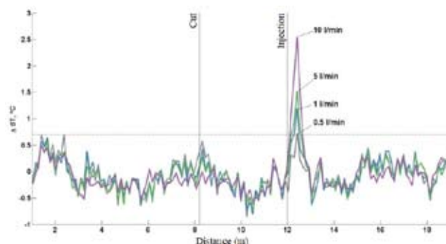
Fig. 5 : Detection parameter during the seepage tests for the Top line. In purple seepage of 10 l×m -1 , in light green seepage of 5 l×m -1 , in dark green seepage 1 l×m -1 and in brown/grey seepage of 0.5 l×m -1 . The first vertical line represents the abscissa at which the puncture simulating the leaks is located, while the second vertical line represents the abscissa at which the water injected below the geomembrane to simulate the seepages is located. The horizontal line represents the threshold above which anomalies can be considered as potential leaks or seepages.
